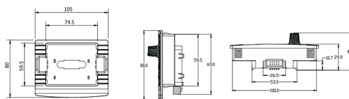
Keyboard base
