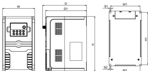
Рис. 3: CV900G-003G-12SF ~ 011G/015P-14TF
