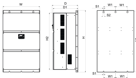
Рис. 10: CV900G-350G/375P ~ 450G/500P-14TF
